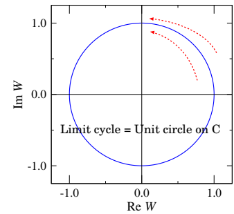
図4 Stuart-Landau 振動子.
